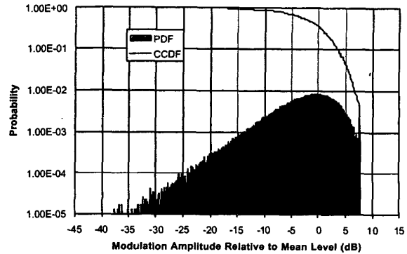
Fig. 3 Probability Distribution of 3GPP Test Model 1 with hard clipping
