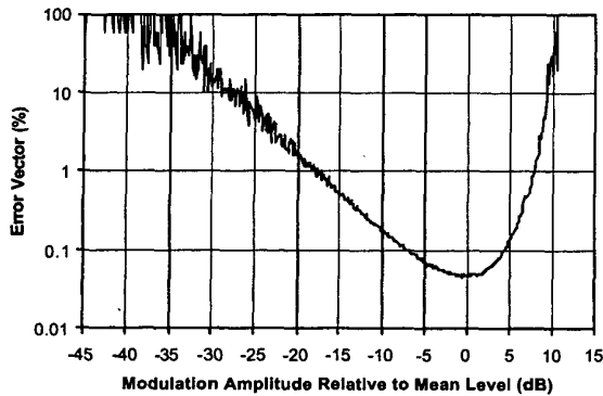
Fig. 2 Modulation Error Vector, weighted according to Test Model 1
